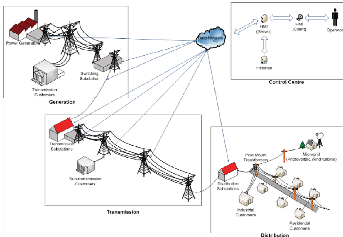
Figure 5: High-level overview of the modern electricity network.
